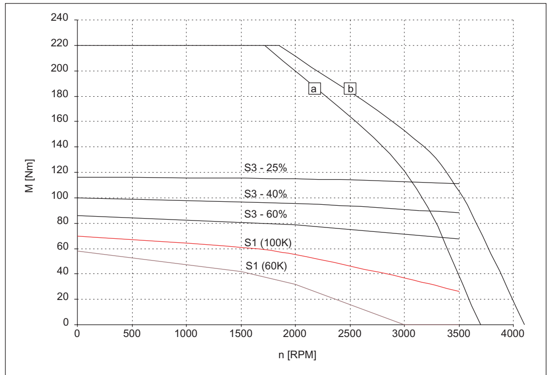
Figure 3-45 Speed-torque diagram 1FT6108-8AF7□
