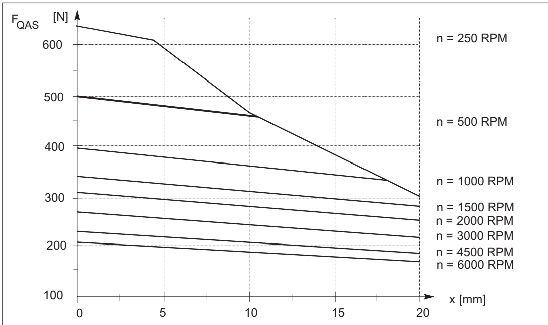
Figure 3-31 Cantilever force F_Q at a distance x from the shaft shoulder for a nominal bearing lifetime of 20,000 h.
