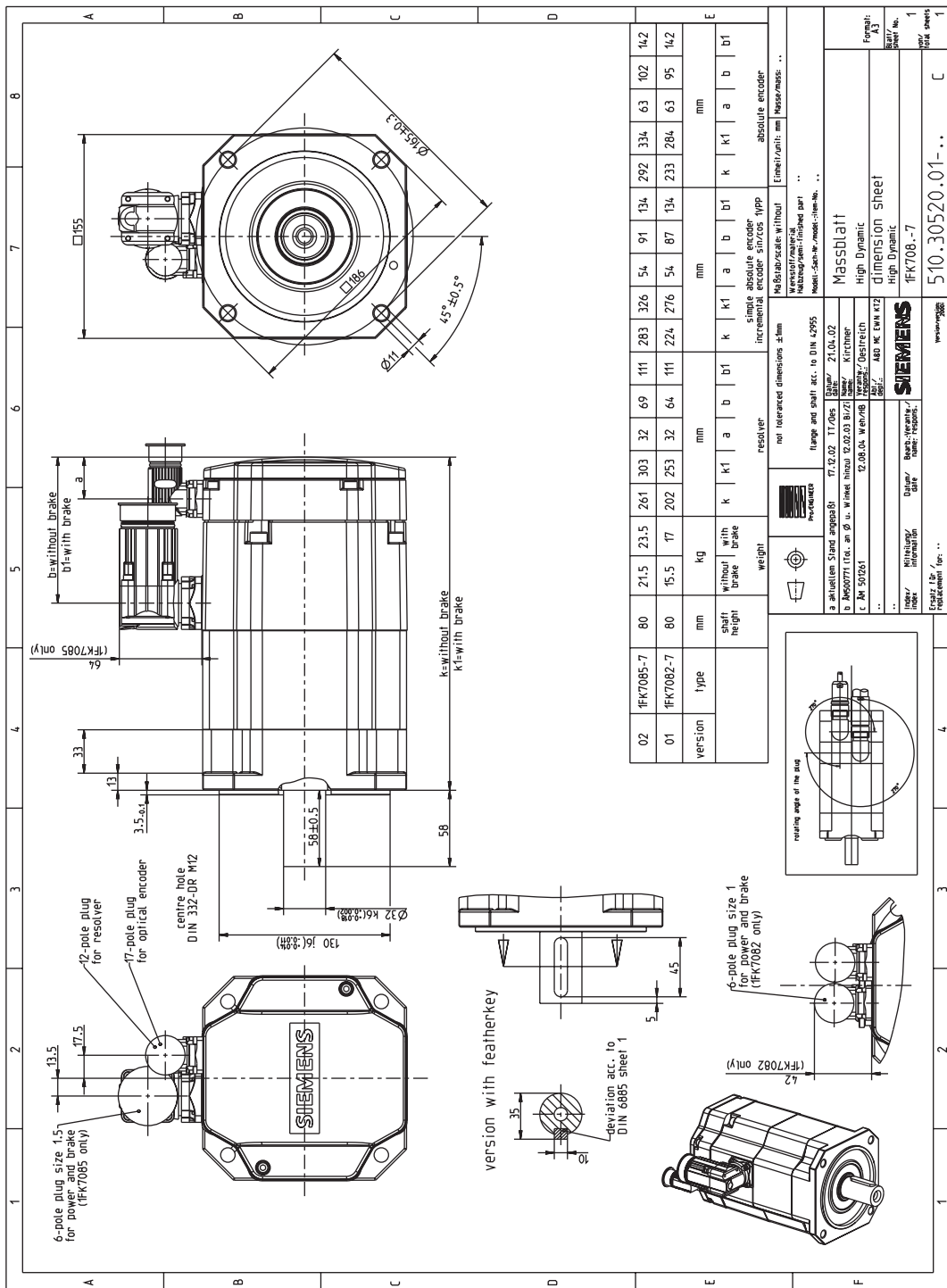
Figure 5-24 1FK708_-7
