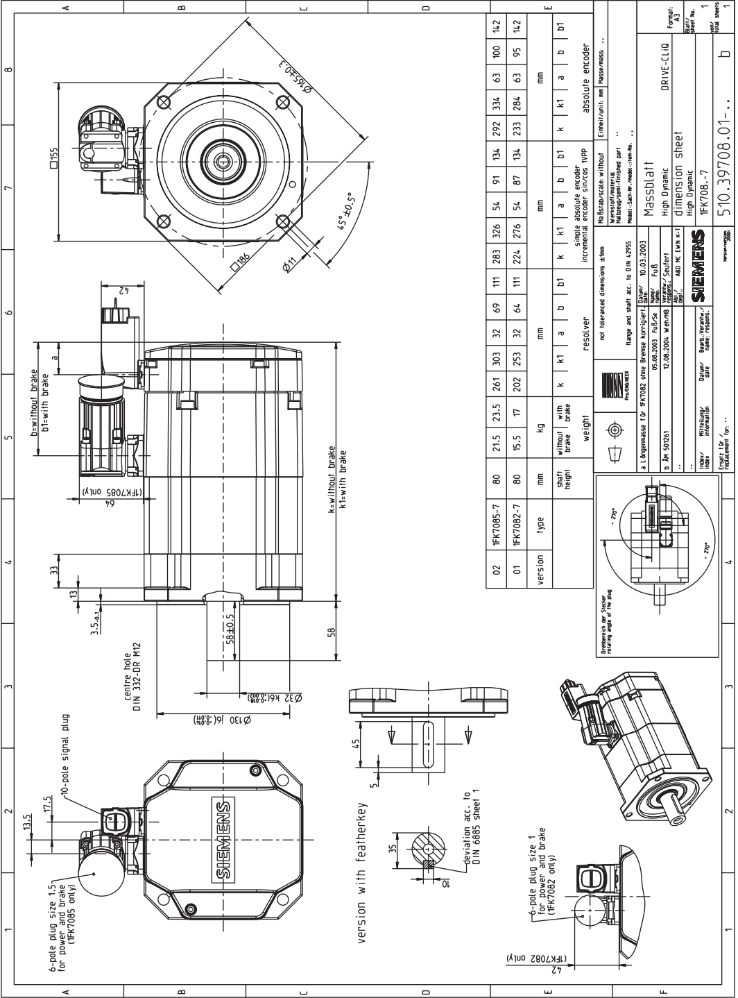
Figure 5-12 1FK7085-7A_DQ
