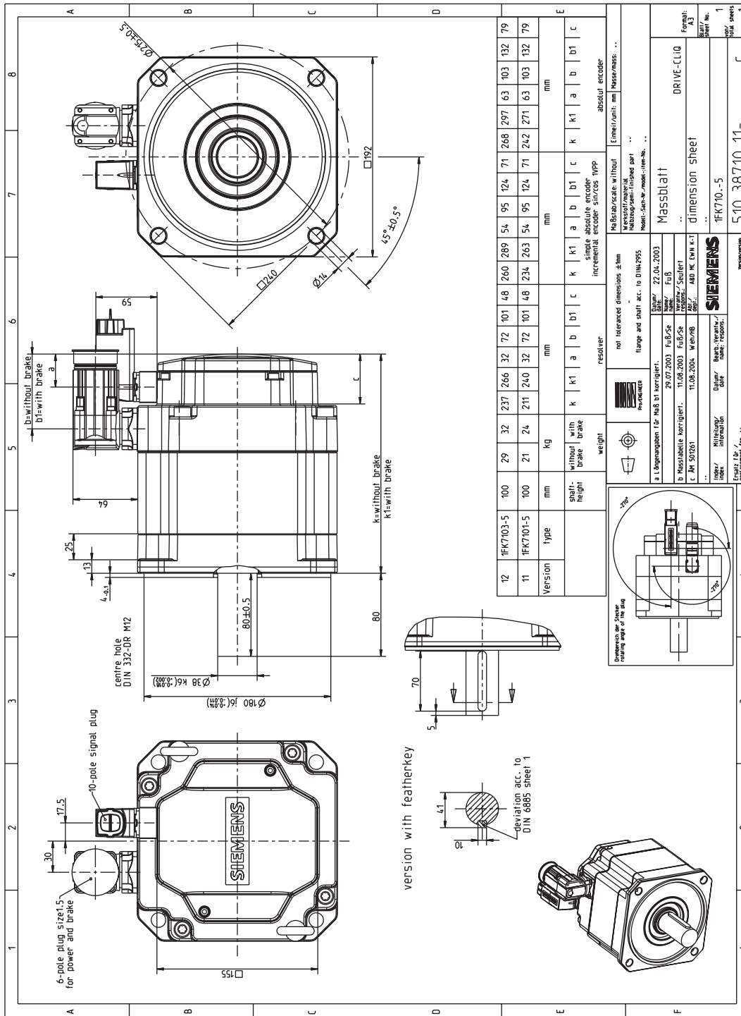
Figure 5-7 1FK7101_1FK7103_5A_DQ
