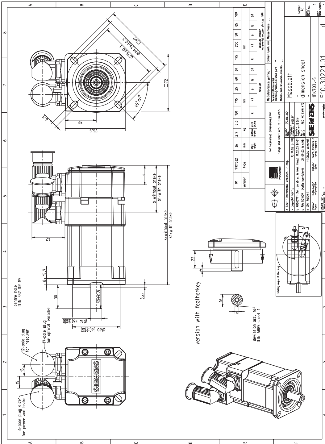
Figure 5-14 1FK703_-5
