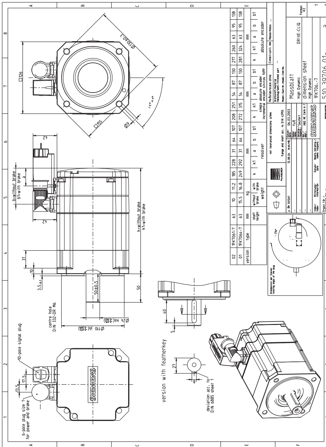
Figure 5-11 1FK706_-7A_DQ
