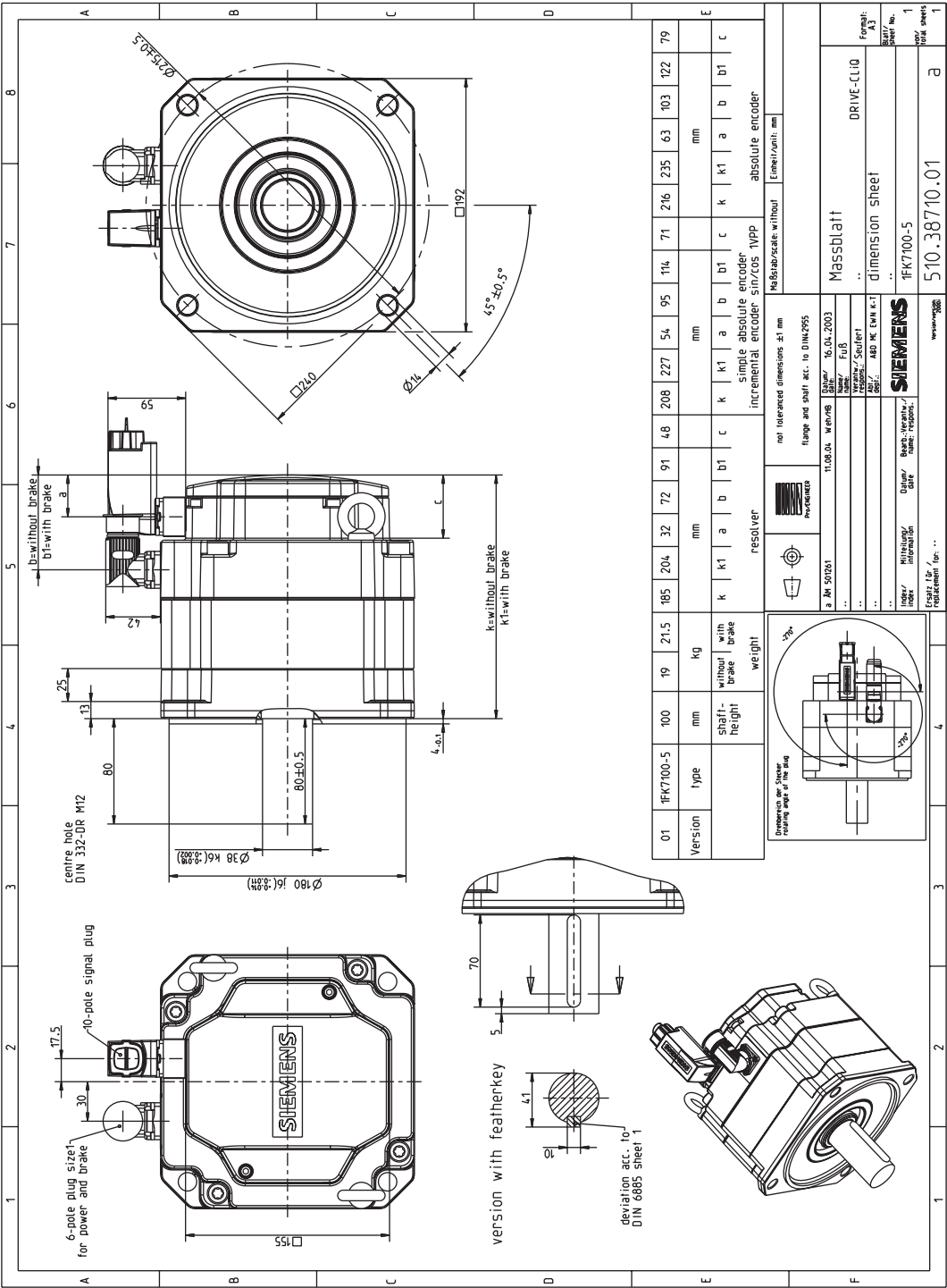
Figure 5-6 1FK7100-5A_DQ
