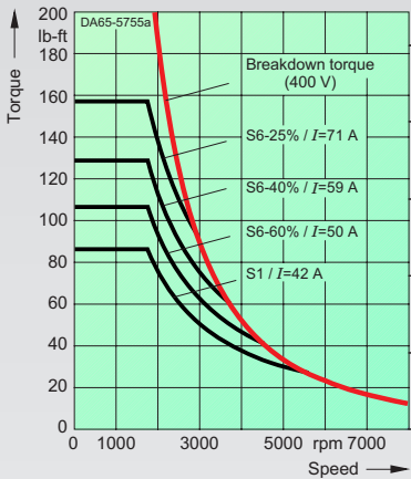
1PH7135-2.F.-..... max. breakdown torque: 258 lb-ft/350 Nm
