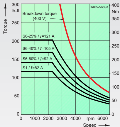
1PH7163-2.G...-.... max. breakdown torque: 496 lb-ft/672 Nm
