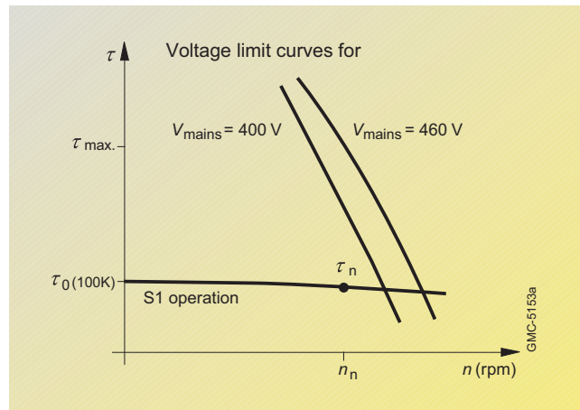
Fig. 2/8 Torque-speed characteristic
