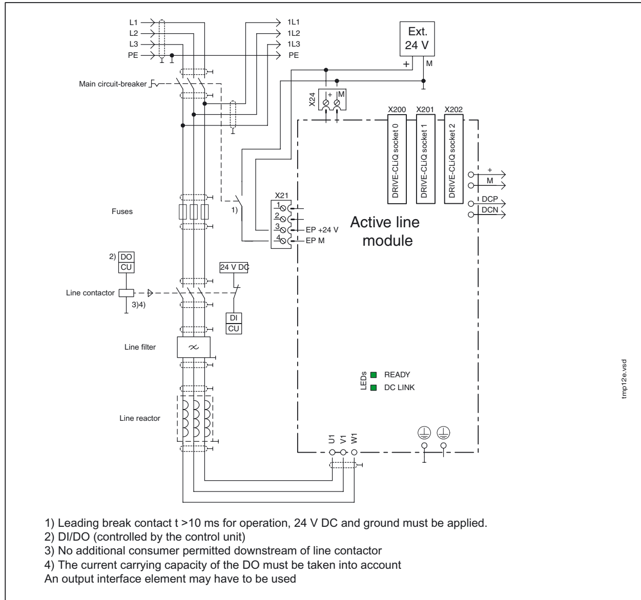
Figure 3-3 Example connection of Active Line Module
